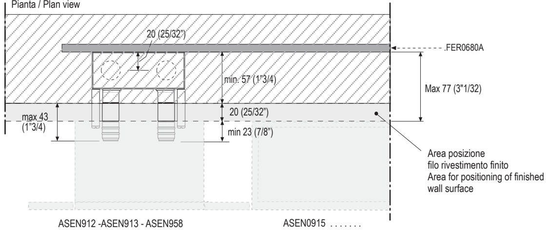
Pianta / Plan view
